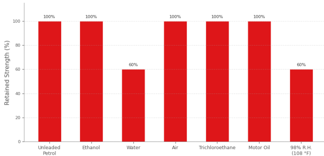
Chemical Resistance — Steel Lap Shear Strength Retention (ASTM D 1002)
